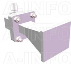
LB-75-10-C-TFSP Standard Gain Horn Antenna 10-15GHz 10dB Gain TNC Female
