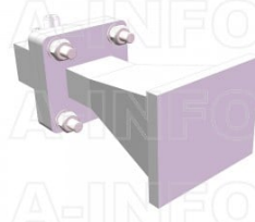
LB-75-10-C-SFSPO Standard Gain Horn Antenna 10-15GHz 10dB Gain SMA Female
